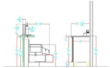
SIDE SECTION ELEVATION FROM FRONT AND BACKBAR EQUIPMENT
